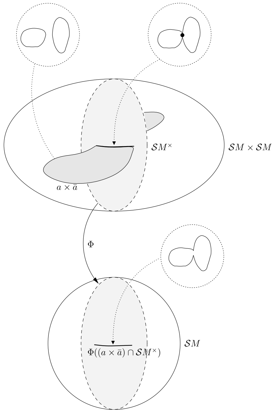
Figure 3: The definition of the string bracket.
