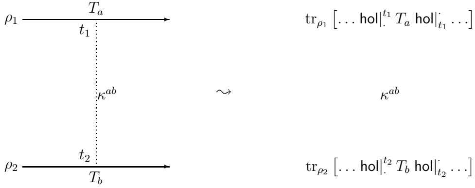
Figure 8: The form \mathfrak{h} associated to (a part of) a chord diagram; t_1 and t_2 refer to a S^1 -parametrization of the circles.
