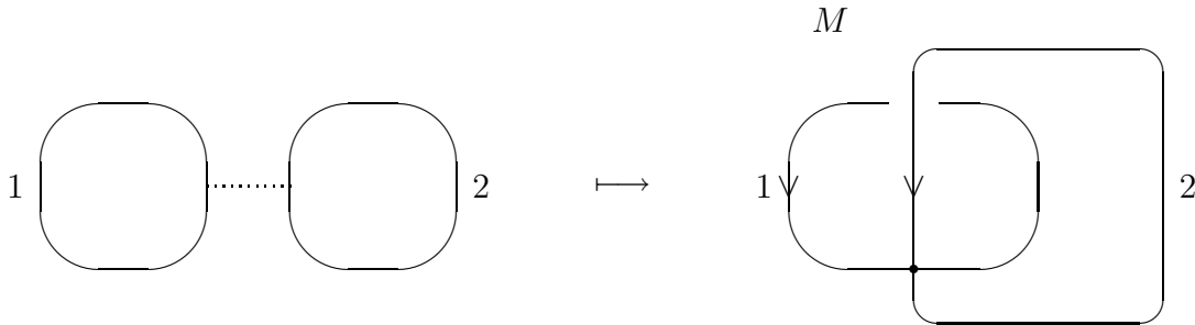
Figure 5: A chord diagram on M .
