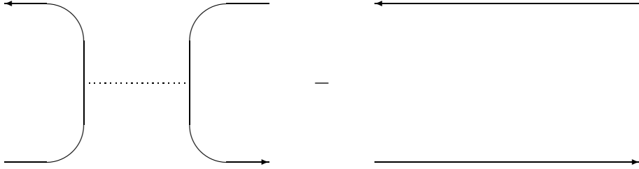
Figure 8: The form \mathfrak{h} associated to (a part of) a chord diagram; t_1 and t_2 refer to a S^1 -parametrization of the circles.
