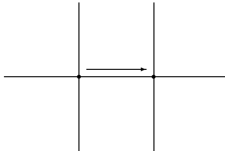
Figure 6: Approaching a boundary on \text{ch}(M) .
