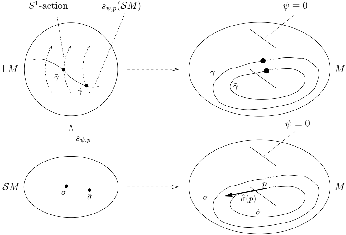
Figure 1: Constructing local coordinates on \mathcal{S}M .
