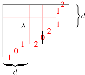
FIGURE 2. The 012-string associated to \lambda and d
